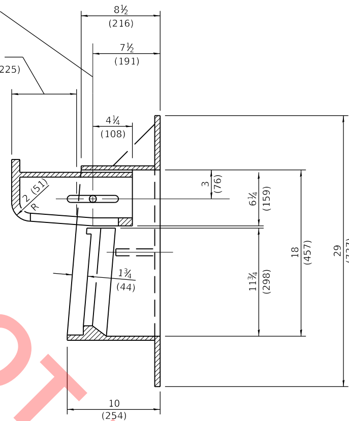
SECTION B-B
