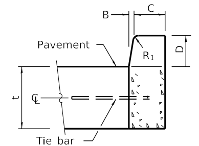
BARRIER CURB
