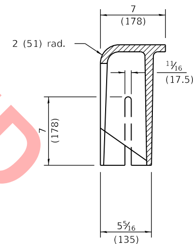
SECTION E-E
