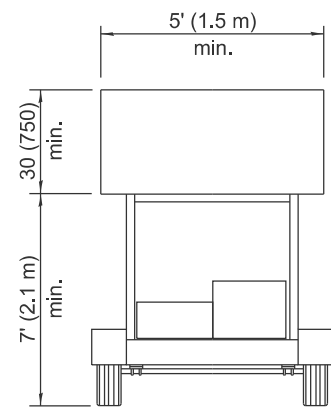
TYPE B ROOF OR TRAILER MOUNTED
