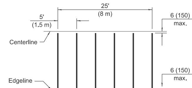
TYPICAL INSTALLATION
