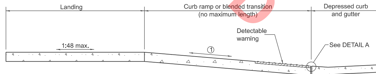
SECTION C-C
