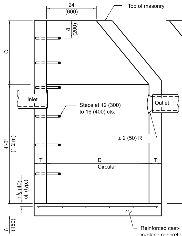
ELEVATION (Standard Outlet)
